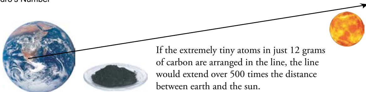
Figure 9.1 Avogadro's Number
